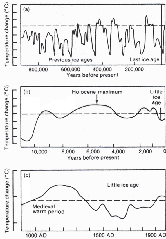
Figure 7.1: Schematic diagrams of global temperature variations since the Pleistocene on three time-scales: (a) the last million years, (b) the last ten thousand years, and (c) the last thousand years. The dotted line nominally represents conditions near the beginning of the twentieth century.
